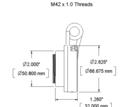
LC-2A-M42 (M42x1-Mount Lens Adapter)
