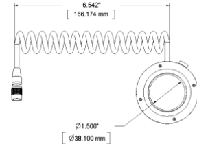
LC-2A-M42 (M42x1-Mount Lens Adapter)
