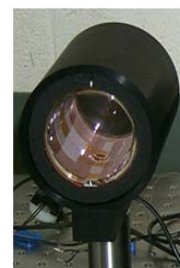
Packaged I2S-5 with integrated thermocouple and heating element in aluminum housing.
