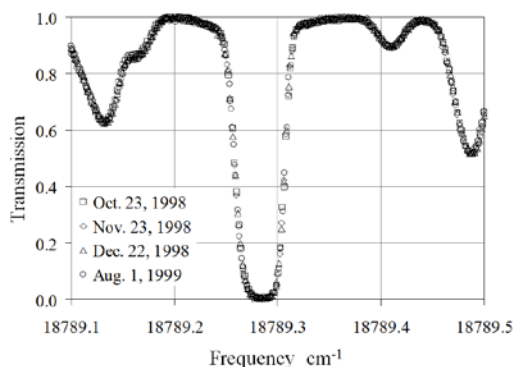
Long term stability of sealed Iodine Cell
