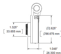
LC-2A-C (C-Mount Lens Adapter)
