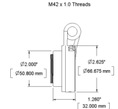
LC-2A-M42 (M42x1-Mount Lens Adapter)
