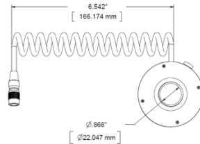
LC-2A-C (C-Mount Lens Adapter)
